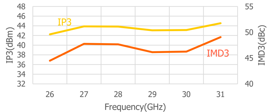
IP3/IMD3 v.s. Freq.
