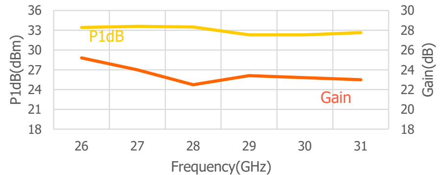
P1dB/Gain v.s. Freq.
